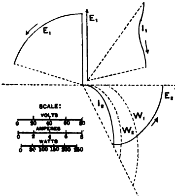
FIG. 17.—Constant Potential, Step Up, Arm at 90°.
